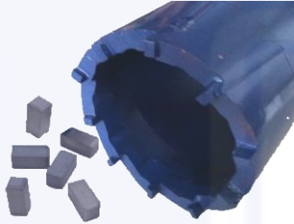
Single Tube Core Bit
