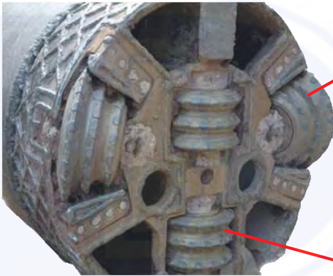
8800 mm Pipe Jacking Cutting Head working at Holland Road, Singapore
