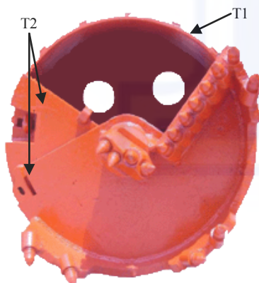
ROCK BUCKET
